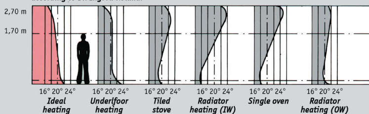
Temperature profiles according to Dr. Ing. A. Kollmar
